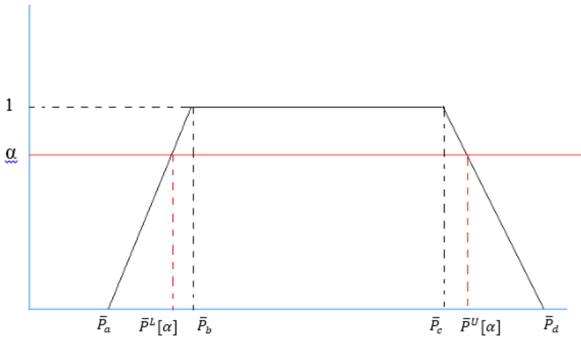
Fig.2- Representation of \alpha -cut fuzzy set \tilde{P}
