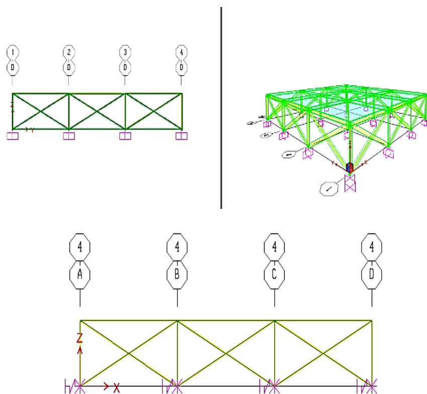
Fig. 3- The 3-D view of the sliding building and the grid consisted of orthogonal girder and its supporting space truss
